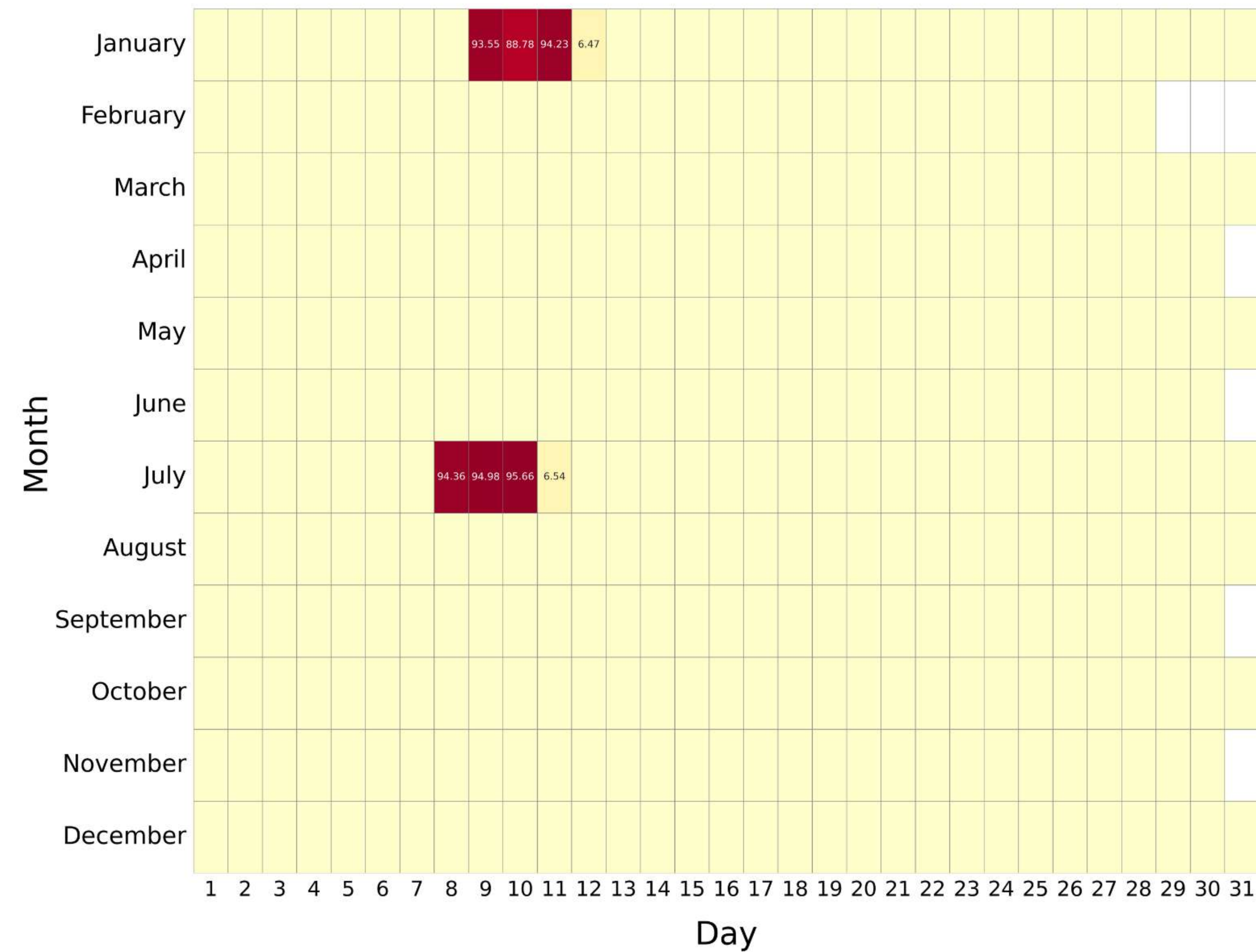
RR:V8 (Temperature) NLC , year: 2011
