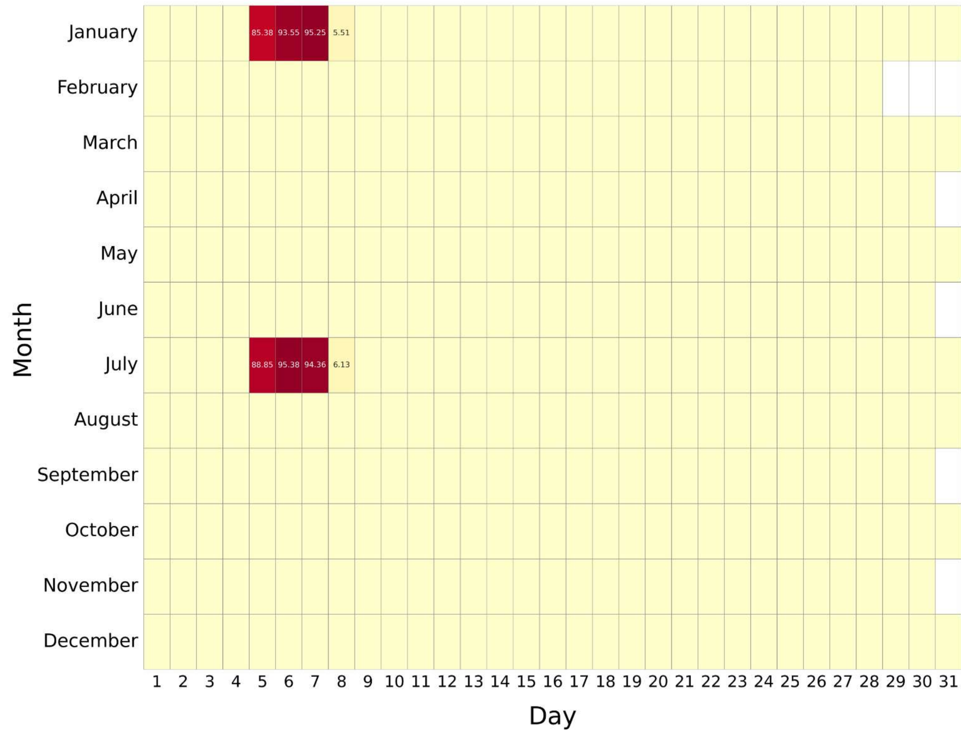
RR:V8 (Temperature) NLC , year: 2011
